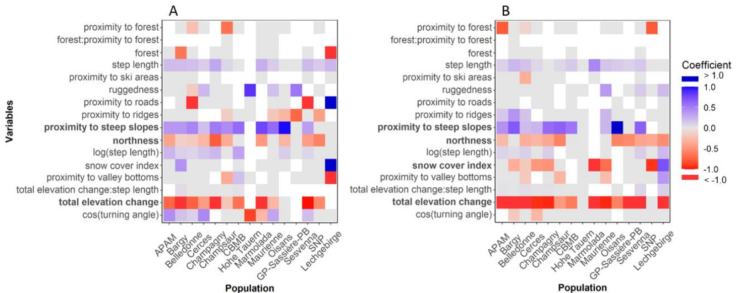
877 Figure 3: Coefficients provided by population-specific model-averaged (models with \Delta AICc < 878 2) integrated Step Selection Analyses investigating the influence of environmental variables on 879 movement steps performed by Alpine ibex from 15 populations during spring (A) or autumn 880 (B) migration. Blue and red cells represent variables that were selected or avoided for migratory 881 movements, respectively. Grey cells represent non-significant coefficients. We calculated the 882 95% confidence interval (CI) of coefficients resulting from the model averaging. A coefficient 883 was significant if its CI non-overlaps with zero. White cells represent cases for which the 884 influence of a focal habitat variable could not be tested (not retained during model selection). 885 A variable name is in bold type if its selection coefficient was significant in at least 8/15 886 populations.
