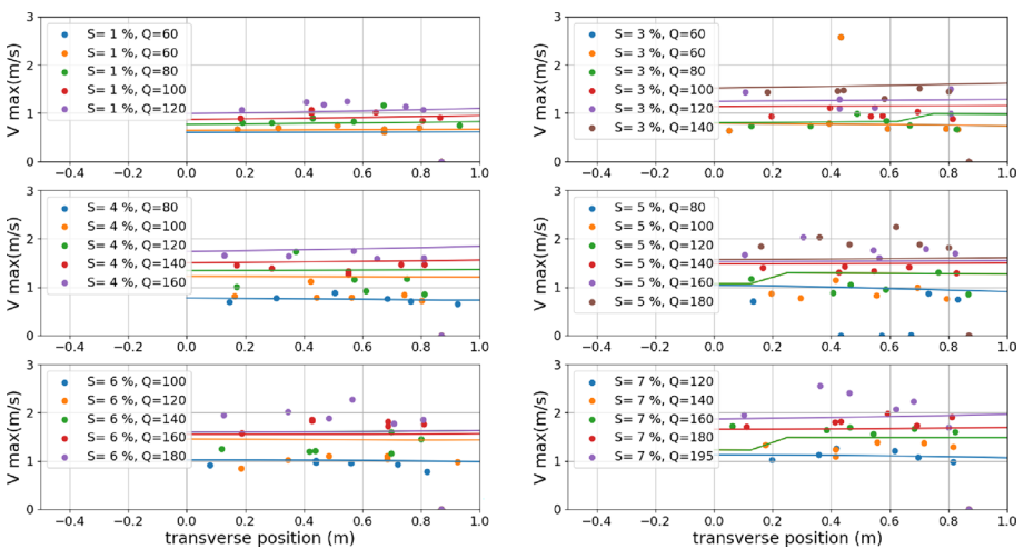
Fig. 17 Cross-sectional profile of maximum measured and calculated velocities for configuration 2. Dots represent measurements and curves are the model [8]
