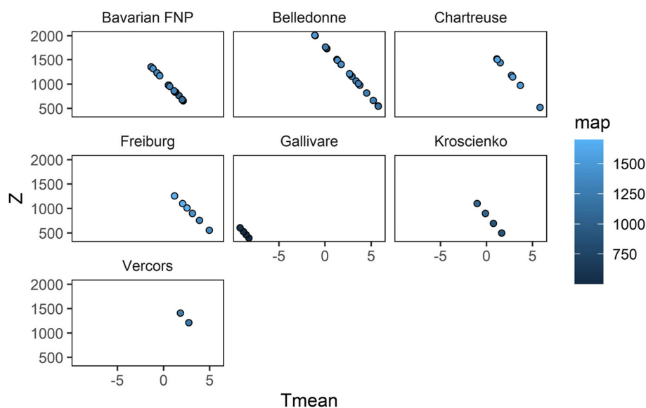
Fig. 4 Mean annual temperature ( T_{\text{mean}} , °C), annual precipitation (map, mm year -1 ) and elevation (Z, m) of the elevation levels in each site
